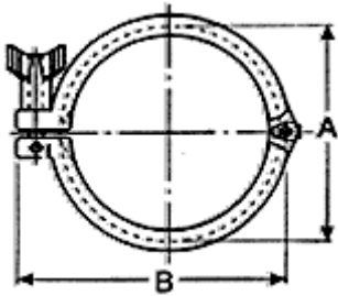
13LAH (13MHH) Single Pin Heavy Duty Clamp
