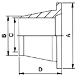
RJT-14 Welding Liner
