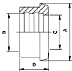
DIN-14R(DIN-11851) Expanding Liner
