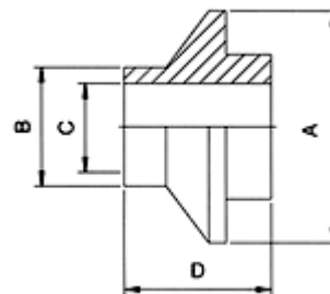
14WI I-Line Short Male Ferrule
