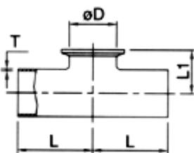
BPE Equal Outlet Tee Weld/ Clamp End (DT-15)
