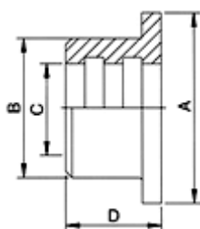
SMS-14R Expanding Liner
