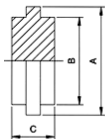
IDF-16 Blank Liner
