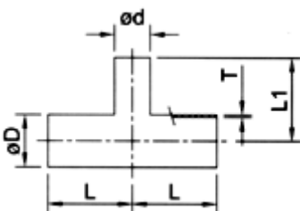
BPE Reducing Tee Weld End (DT-10)
