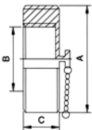
RJT-13RBN Round Blank Nut
