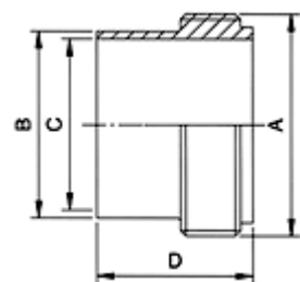
IDF-15L Long Welding Male
