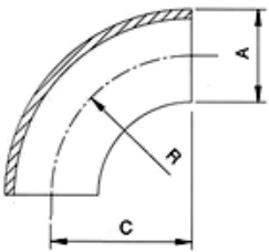
2WC 90° Short Elbow
