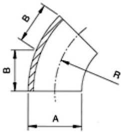
2KW 45° Short Elbow
