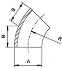
SMS 45° Short Elbow
