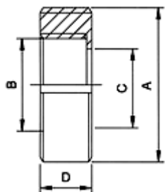
DIN-13RI(DIN-11851) Round Nut 4 Slots
