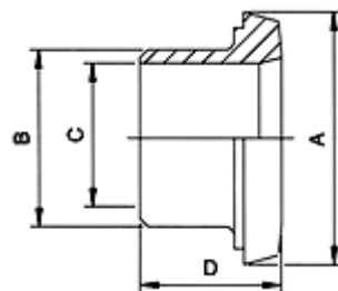
DIN-14I(DIN-11851) Imperial Welding Liner
