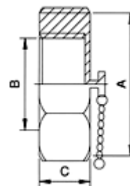
RJT-13HBN Hex. Blank Nut
