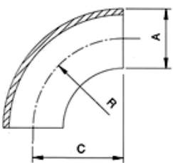
SMS 90° Short Elbow
