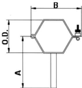
THHP Tube Hanger With Pipe
