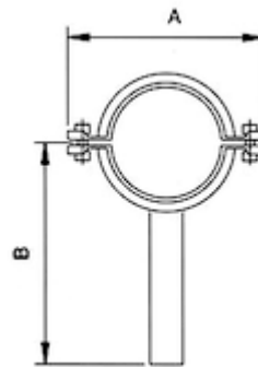
THRL Tube Hanger Long Type
