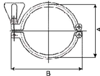
13MHHA L.B. Double Pin Heavy Duty Clamp
