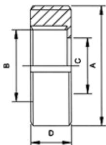
DIN-13R(DIN-11851) Round Nut 4 Slots
