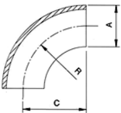
BS 90° Short Elbow
