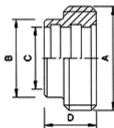
DANSK-15R Expanding Male Part
