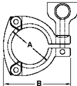
13MHHS 3-Piece Segmental Clamp
