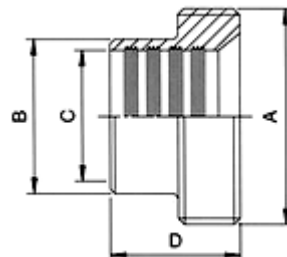
15R Expanding Liner
