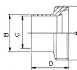
DIN-15(DIN-11851) Welding Male
