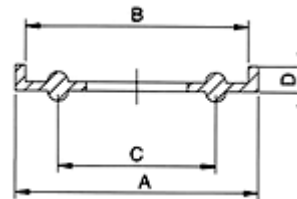
Seal For Ferrule Lipped Type (Type 2)
