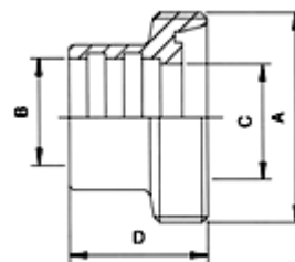
DIN-15R(DIN-11851) Expanding Male
