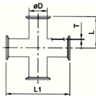
BPE Equal Cross Clamp End (DT-18)
