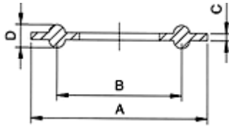
Seal For Ferrule Plain Type (Type 1)
