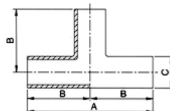
BS Welding Long Tee
