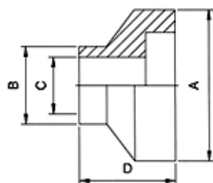
15WI I-Line Short Female Ferrule
