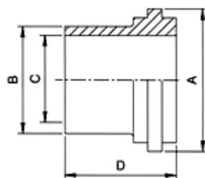
IDF-14L Long Welding Liner
