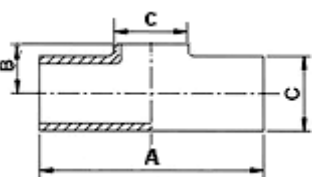
BS Tee Without Straight-End
