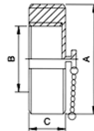
IDF-13HRBN Round Blank Nut
