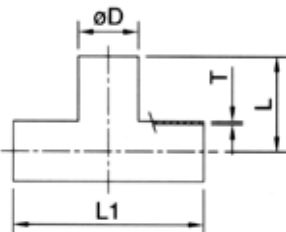
BPE Reducing Tee Weld End (DT-10)
