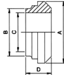
14A Long Weld Liner
