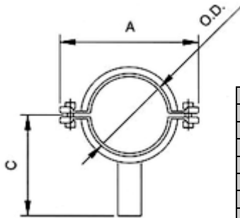
THRS Tube Hanger Short Type
