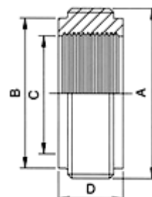
IDF-15R Expanding Male
