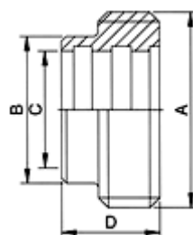
SMS-15R Expanding Male
