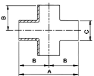
9WWW Short Equal Cross
