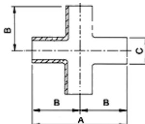
BS Long Cross
