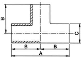
BS Welding Short Tee
