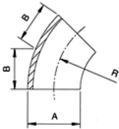
BS 45° Short Elbow
