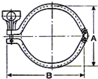
13MHM Double Pin Heavy Duty Clamp
