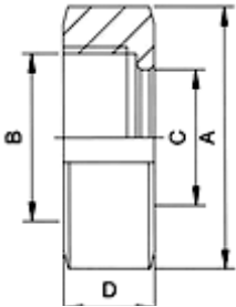
RJT-13R Round Nut 6 Slots
