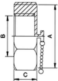
IDF-13HBN Blank Nut
