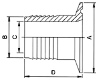
14MPHR Hose Adapter Ferrule
