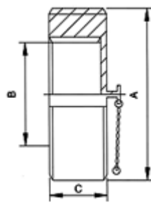
DIN-13RBN(DIN-11851) Round Blank Nut
